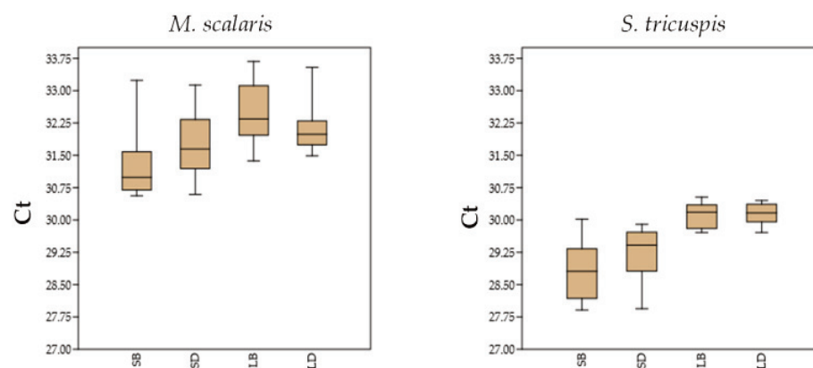
Figure 3. Distribution of the Ct values observed at LOD for M. scalaris and S. tricuspsis isolate materials for the small-scale DNA extraction from honeybees (SB) and hive debris (SD) and the large-scale DNA extraction from honeybees (LB) and hive debris (LD).
