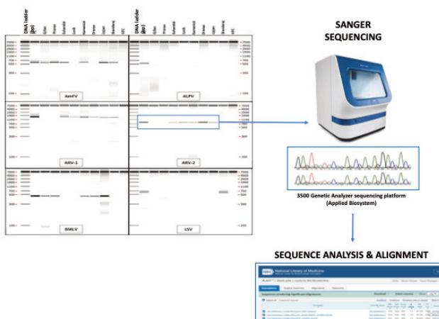
Figure 2. Capillary electrophoresis on LabChip GX Touch HT* of the PCR products for the six emerging honey bee viruses (AmFV, ALPV, ARV-1, ARV-2, BMLV and LSV). DNA ladder: from 100 to 7000 bp; PC: PCR positive control; NTC: PCR negative control. On the lower right, the results of alignment of ARV-2 sequences with those available in the GenBank database using BLAST.
